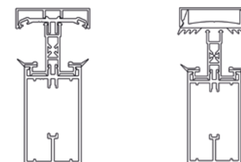
22 Fit hip and transom pressure plates centrally on the rafter (hips will locate into the central channel on the rafter). Ensure that pressure plates are pushed up against the side of the ridge topcap.
